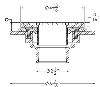
Center Drain
